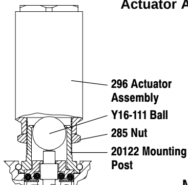
Model 206-C & 206-2-C Pilot Actuated
