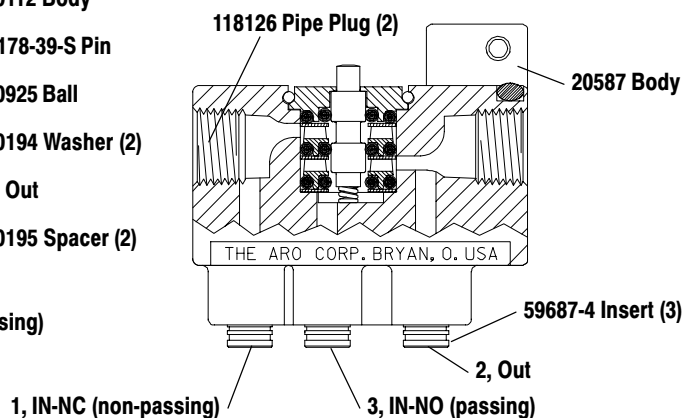
Model 20(-)-2-C 5/32" Tubing Ports
