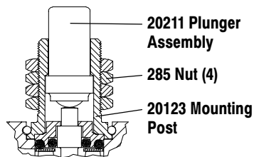
Model 214-C & 214-2-C Straight Plunger
