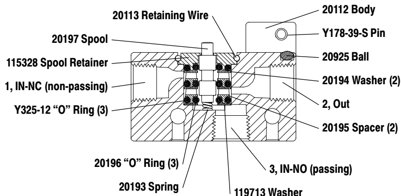
Model 20(-)-C 1/8" NPTF Ports
