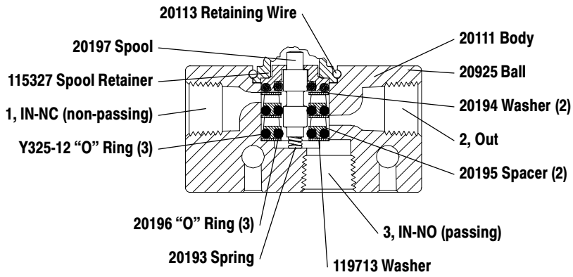
Model 2( )(-C 1/8" NPTF Ports
