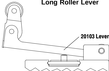
Model 205-C & 205-2-C One-Way, Long Lever
