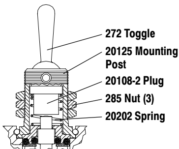
Model 222-C & 222-2-C Centering Toggle
