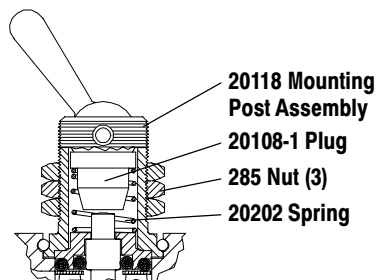
Model 223-C & 223-2-C Retained Toggle
