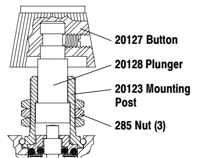
Model 224-C & 224-2-C Panel Button
