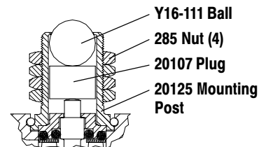
Model 213-C & 213-2-C Long Ball Roller
