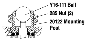
Model 212-C & 212-2-C Short Ball Roller
