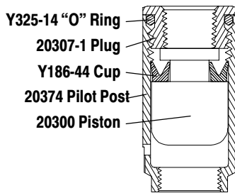
Model 296 Actuator Assembly
